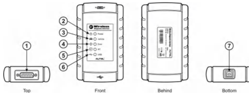
Figure 2-4 Wireless Diagnostic Interface – for MaxiCOM
